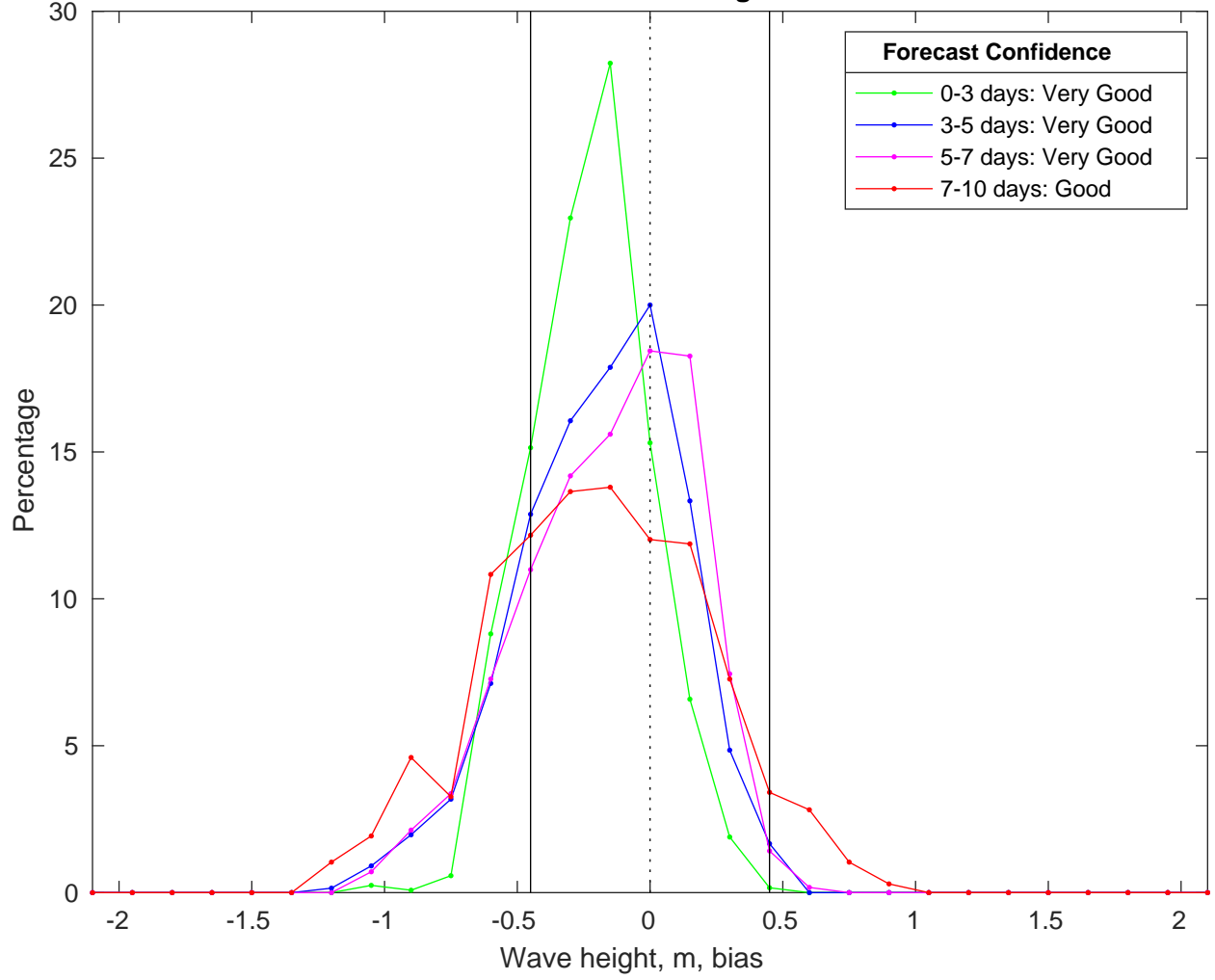
NDBC 52213 vs CMEMS Waves Bias Histogram: 28-Feb-2025
