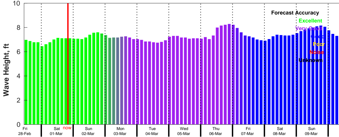
CMEMS Wave Forecast for NDBC 52213 from 27-Feb-2025 11:00:00 to 09-Mar-2025 11:00:00
