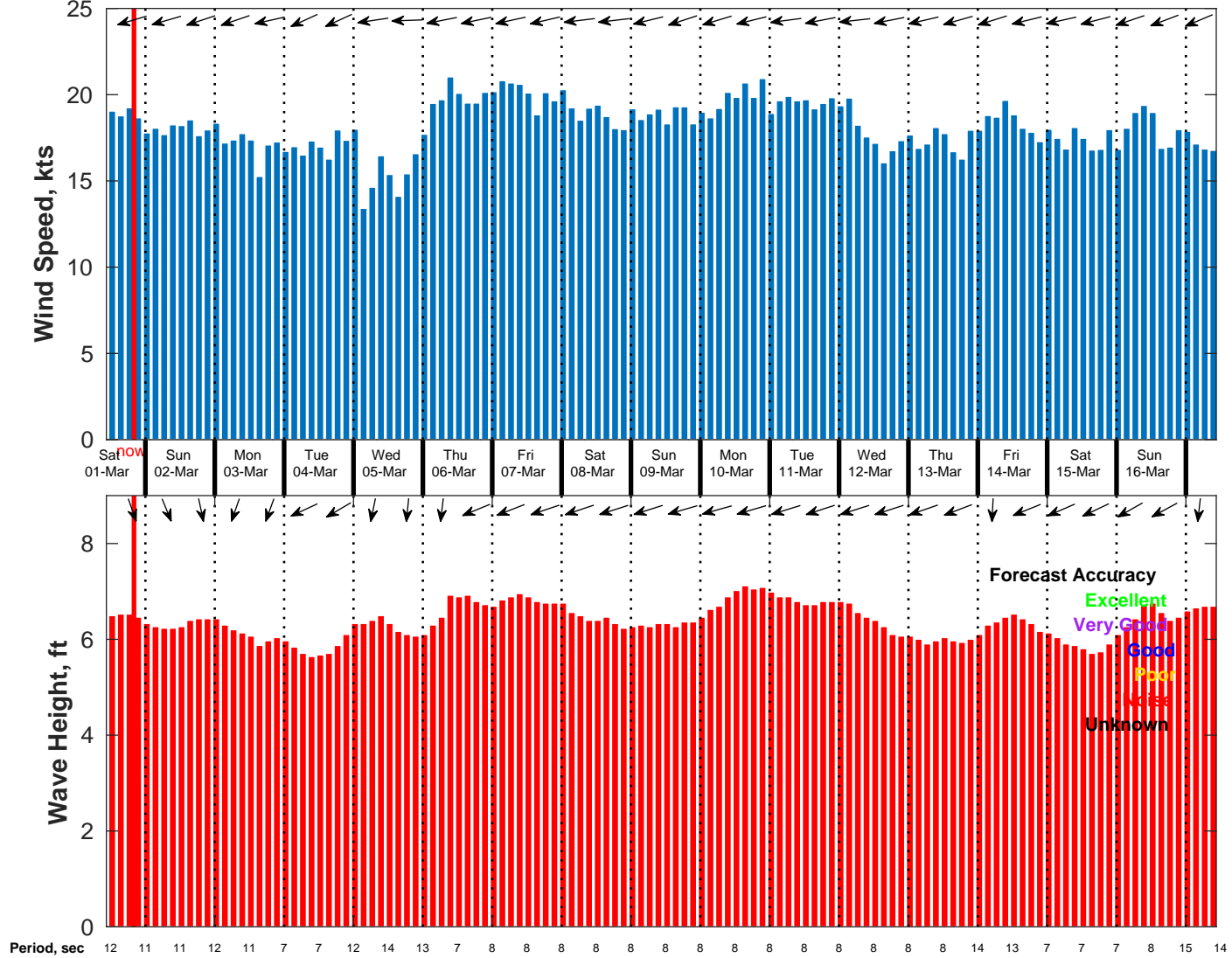
Wind & Wave Forecast for NDBC 52213 from 28-Feb-2025 11:00:00 to 16-Mar-2025 11:00:00
