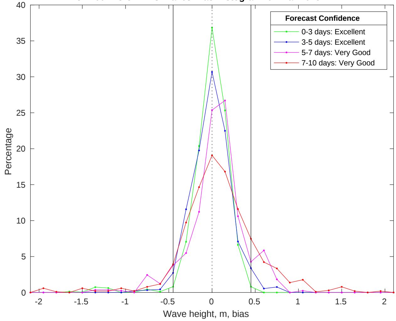
NDBC 41004 vs CMEMS Waves Bias Histogram: 01-Mar-2025
