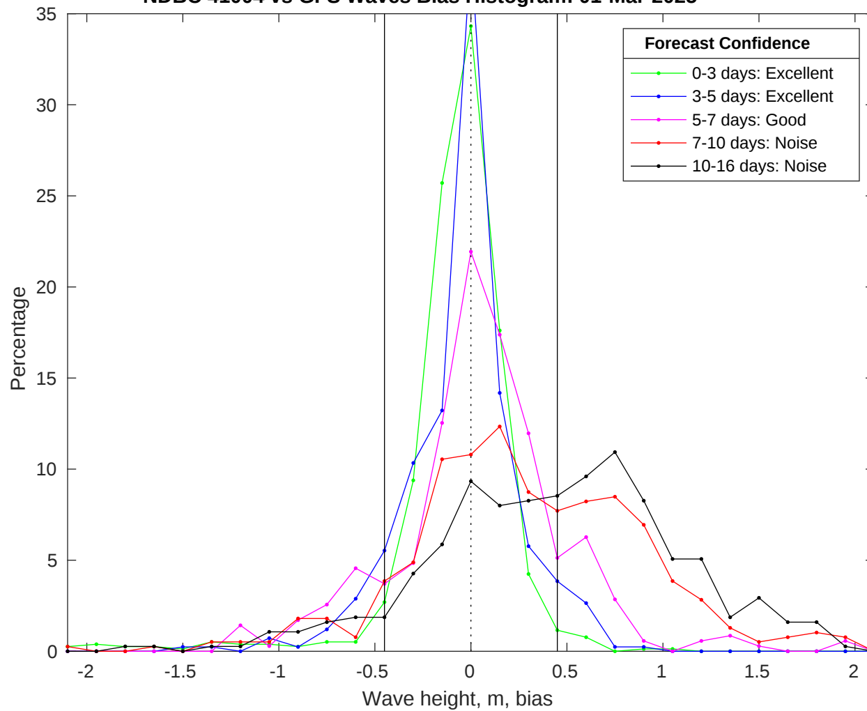
NDBC 41004 vs GFS Waves Bias Histogram: 01-Mar-2025
