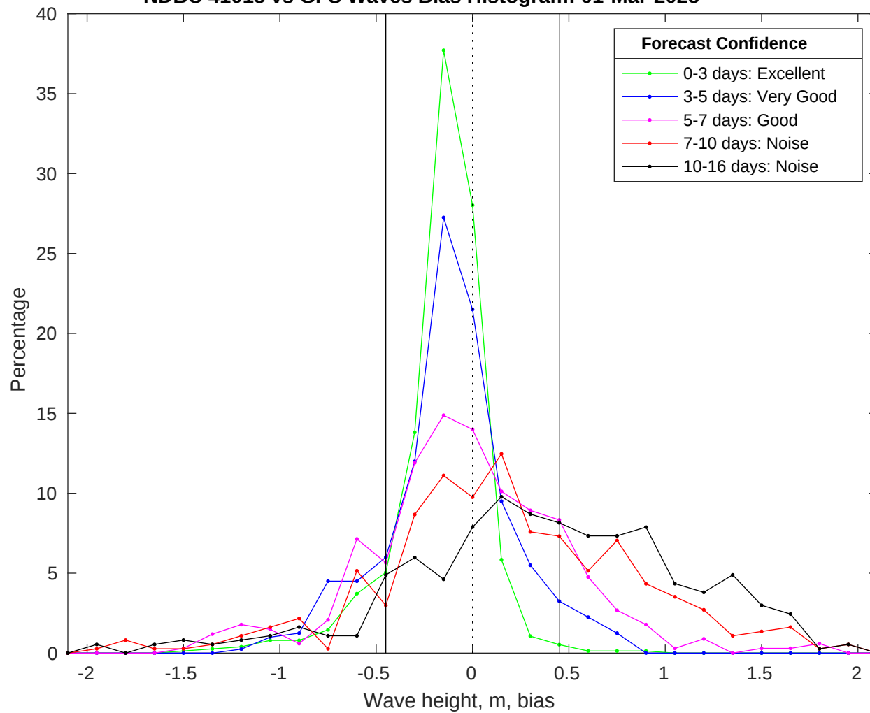
NDBC 41013 vs GFS Waves Bias Histogram: 01-Mar-2025
