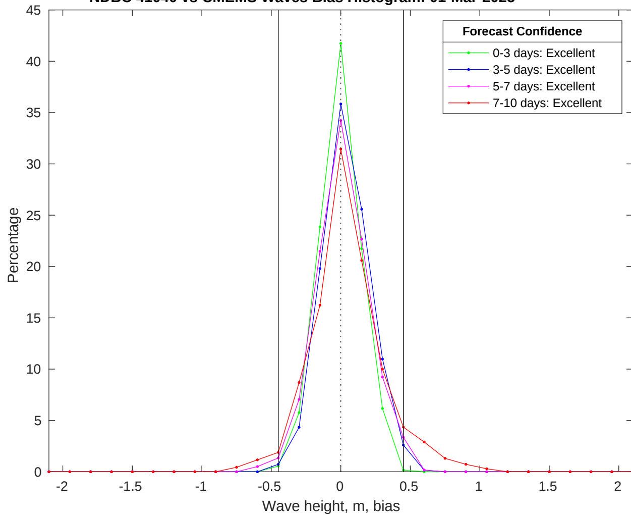
NDBC 41040 vs CMEMS Waves Bias Histogram: 01-Mar-2025
