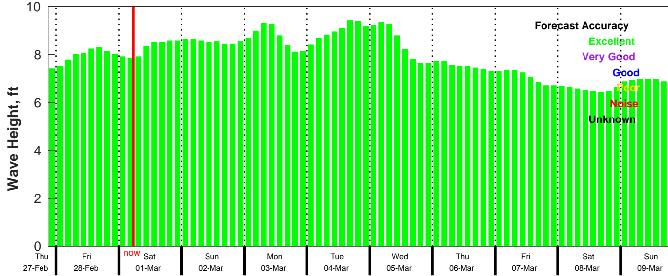
CMEMS Wave Forecast for NDBC 41040 from 27-Feb-2025 21:00:00 to 09-Mar-2025 21:00:00
