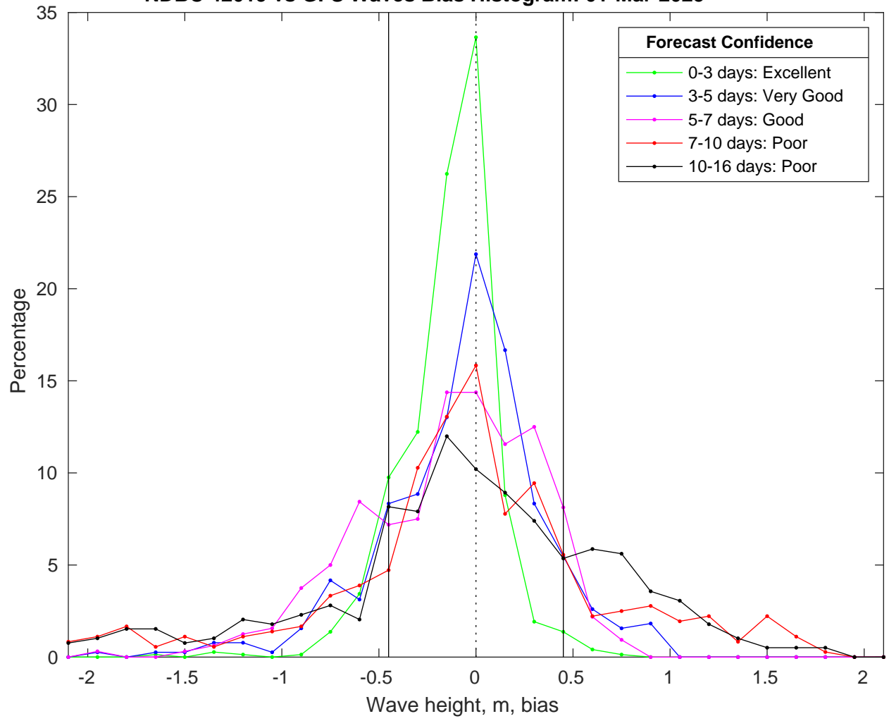
NDBC 42019 vs GFS Waves Bias Histogram: 01-Mar-2025
