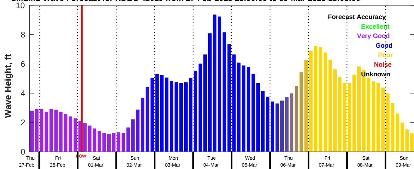
CMEMS Wave Forecast for NDBC 42019 from 27-Feb-2025 18:00:00 to 09-Mar-2025 18:00:00
