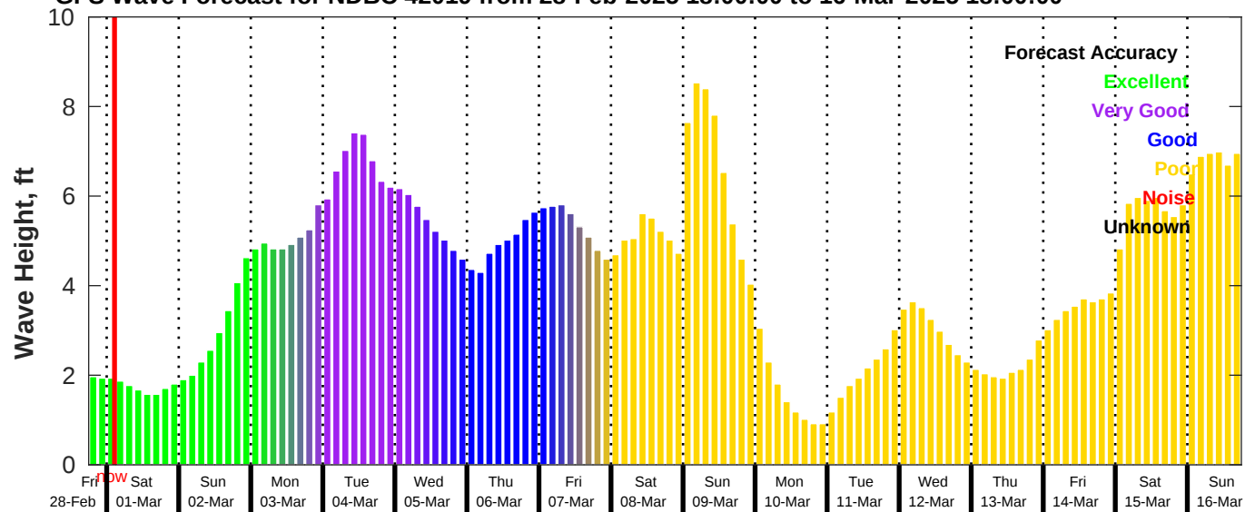
GFS Wave Forecast for NDBC 42019 from 28-Feb-2025 18:00:00 to 16-Mar-2025 18:00:00
