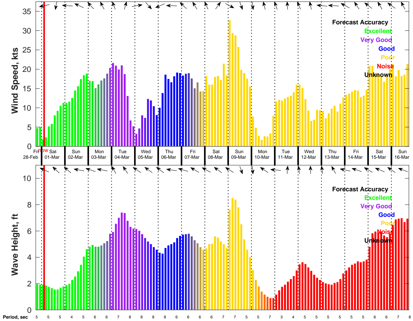
Wind & Wave Forecast for NDBC 42019 from 28-Feb-2025 18:00:00 to 16-Mar-2025 18:00:00
