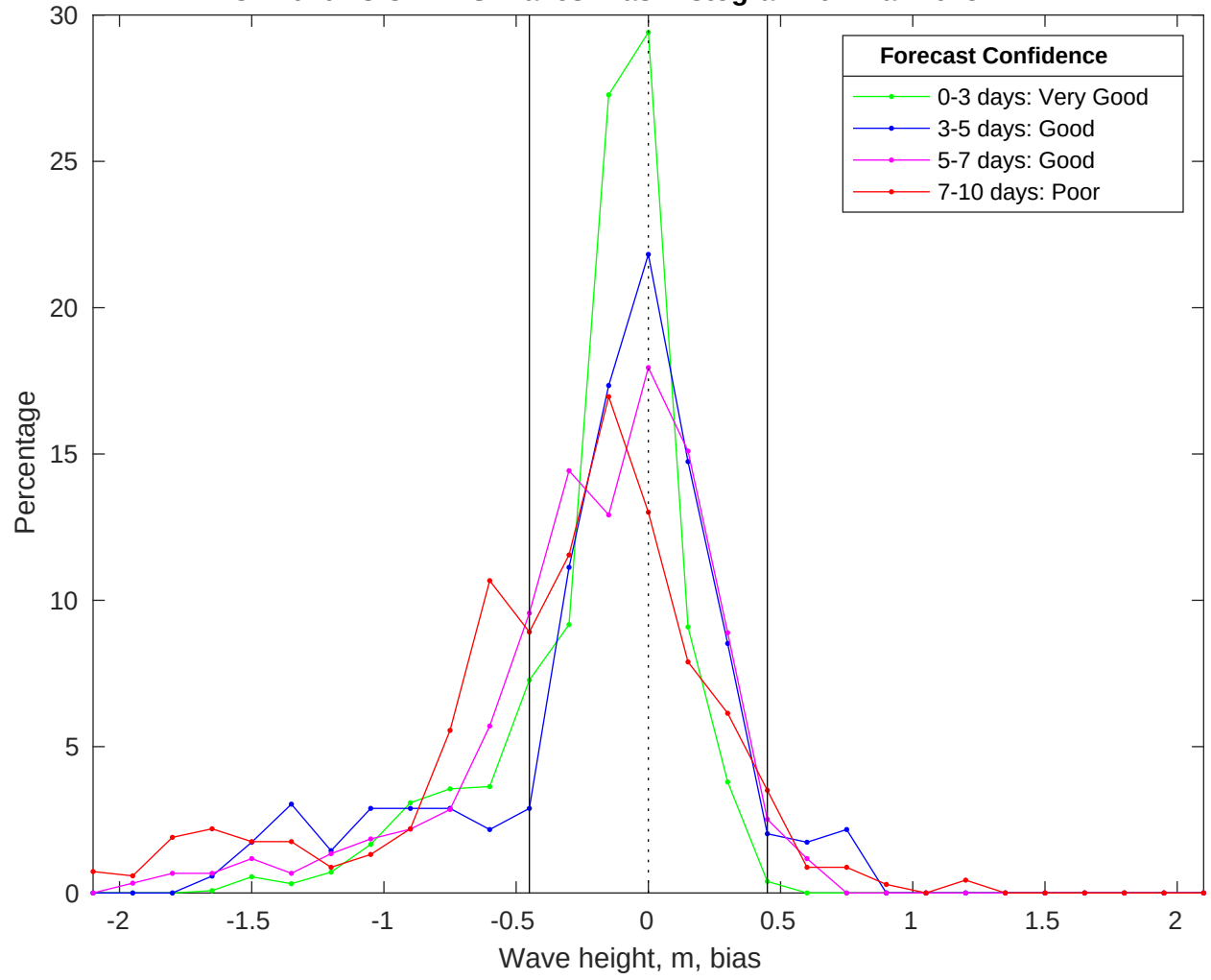
NDBC 42020 vs CMEMS Waves Bias Histogram: 01-Mar-2025
