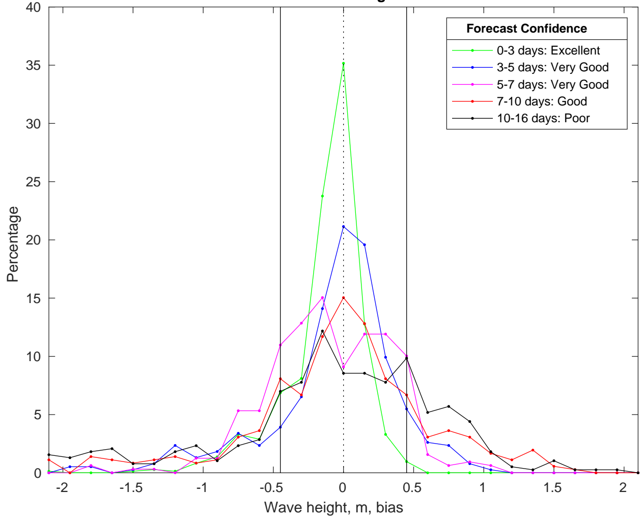
NDBC 42020 vs GFS Waves Bias Histogram: 01-Mar-2025
