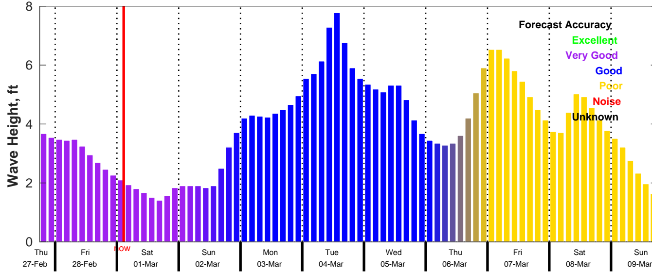
CMEMS Wave Forecast for NDBC 42020 from 27-Feb-2025 18:00:00 to 09-Mar-2025 18:00:00
