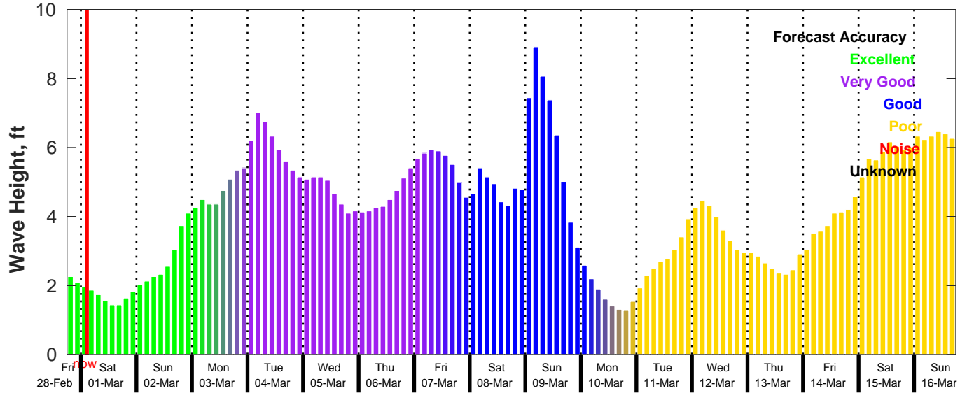
GFS Wave Forecast for NDBC 42020 from 28-Feb-2025 18:00:00 to 16-Mar-2025 18:00:00
