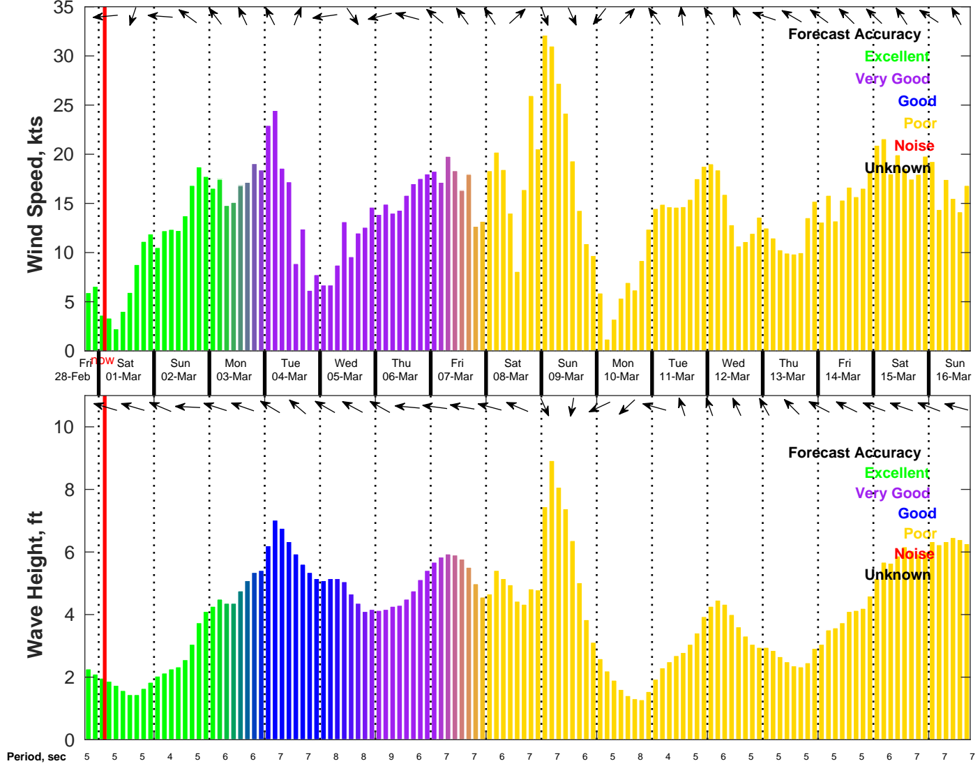
Wind & Wave Forecast for NDBC 42020 from 28-Feb-2025 18:00:00 to 16-Mar-2025 18:00:00
