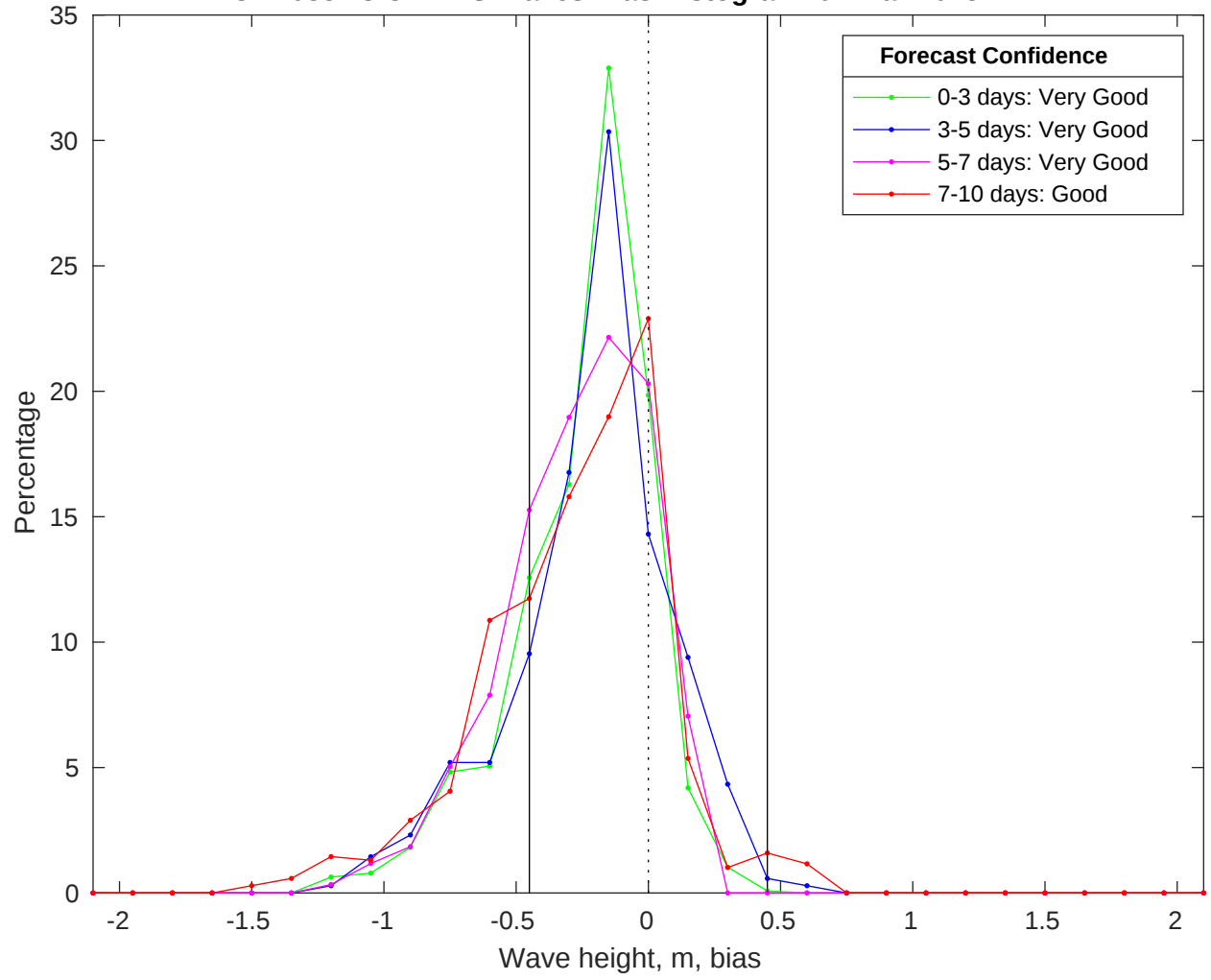
NDBC 42035 vs CMEMS Waves Bias Histogram: 01-Mar-2025
