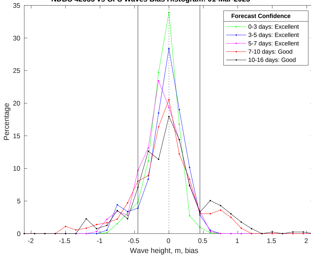
NDBC 42035 vs GFS Waves Bias Histogram: 01-Mar-2025
