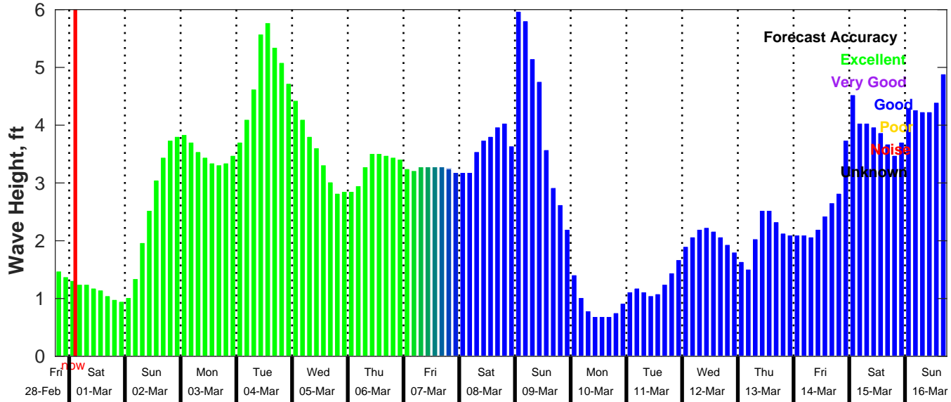
GFS Wave Forecast for NDBC 42035 from 28-Feb-2025 18:00:00 to 16-Mar-2025 18:00:00
