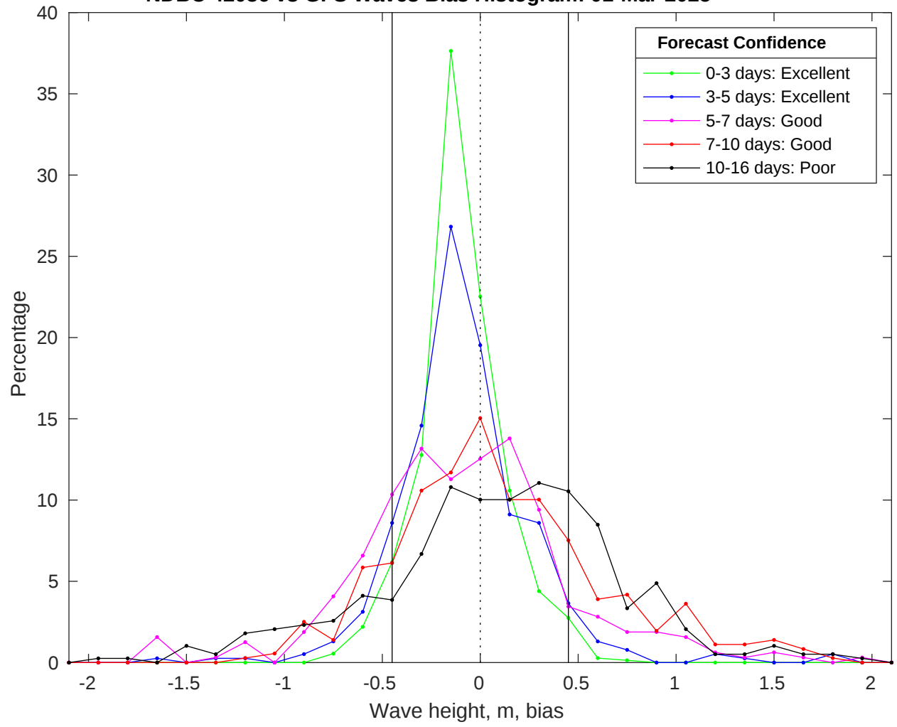
NDBC 42036 vs GFS Waves Bias Histogram: 01-Mar-2025
