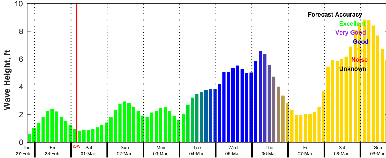
CMEMS Wave Forecast for NDBC 42036 from 27-Feb-2025 19:00:00 to 09-Mar-2025 19:00:00
