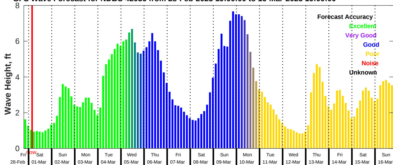
GFS Wave Forecast for NDBC 42036 from 28-Feb-2025 19:00:00 to 16-Mar-2025 19:00:00
