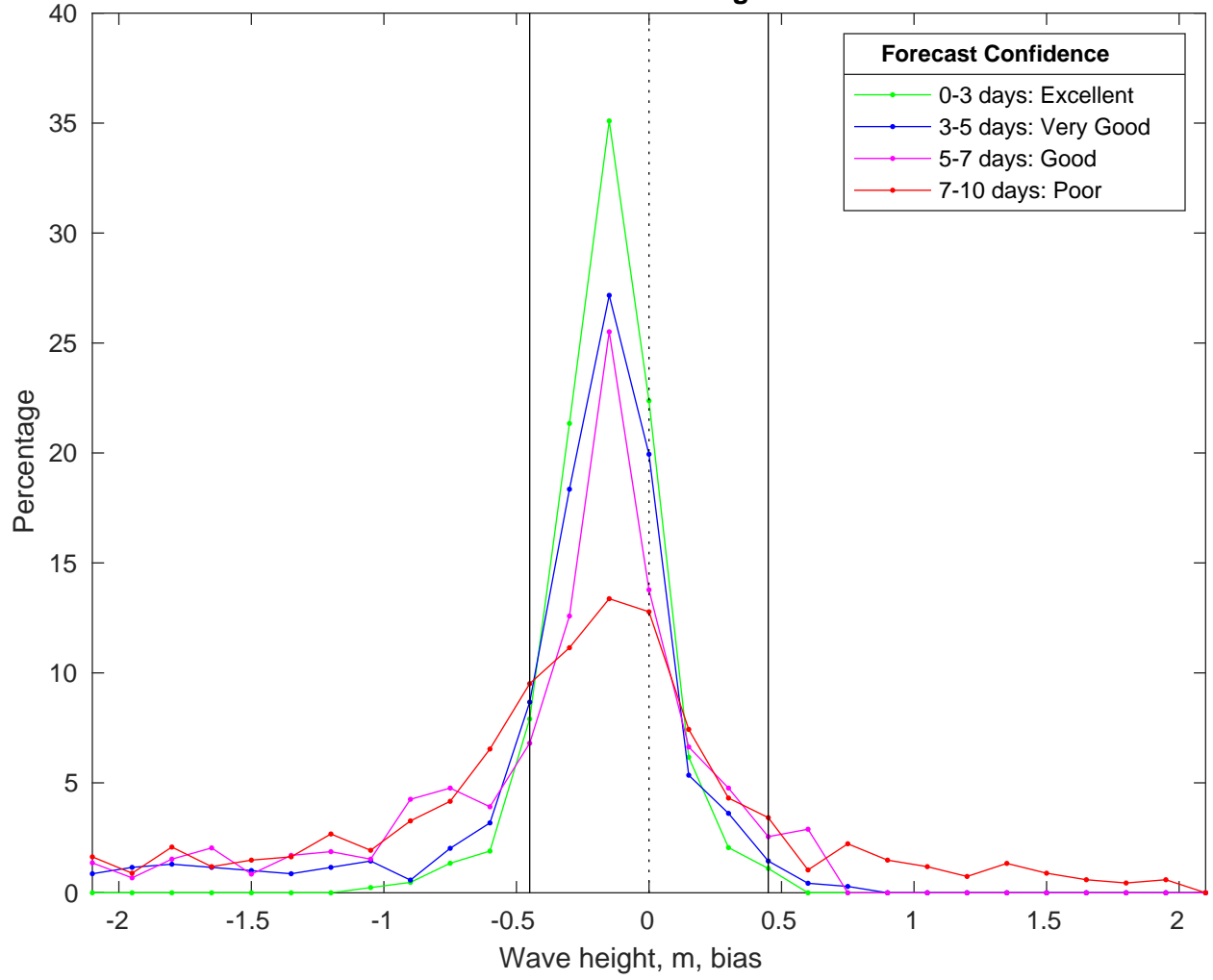
NDBC 42040 vs CMEMS Waves Bias Histogram: 01-Mar-2025
