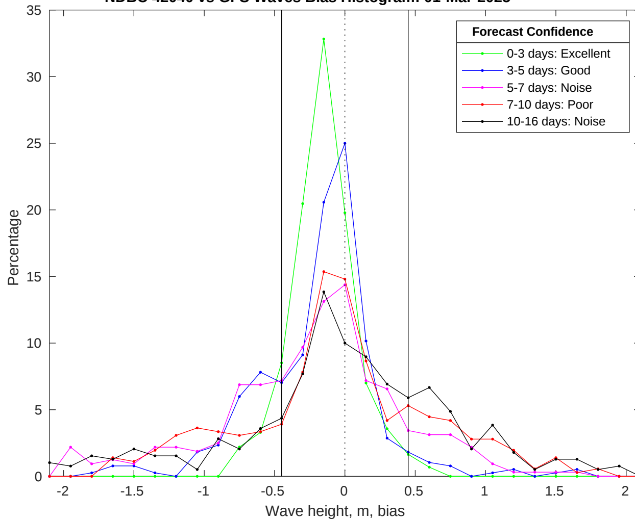
NDBC 42040 vs GFS Waves Bias Histogram: 01-Mar-2025
