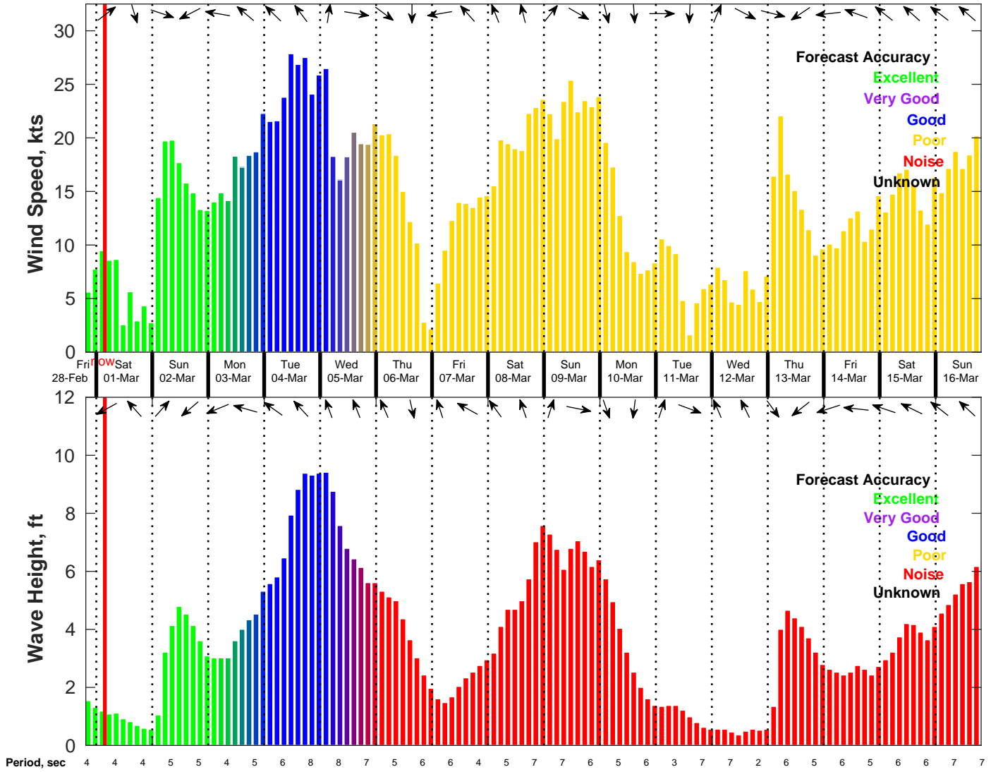
Wind & Wave Forecast for NDBC 42040 from 28-Feb-2025 19:00:00 to 16-Mar-2025 19:00:00
