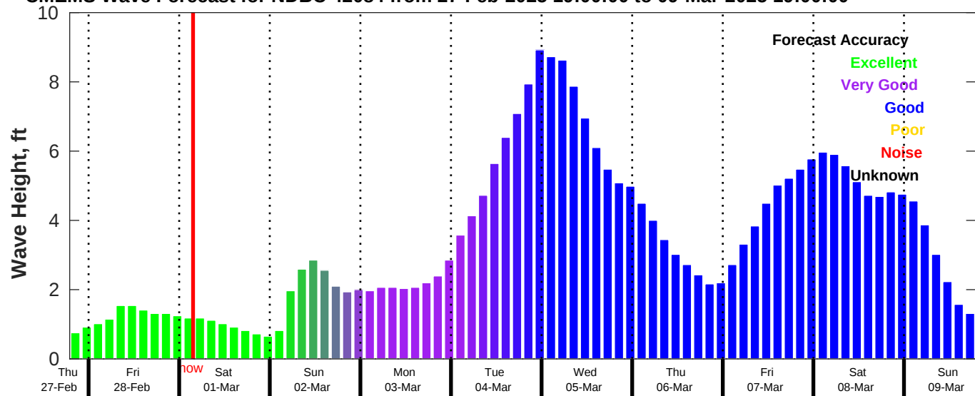
CMEMS Wave Forecast for NDBC 42084 from 27-Feb-2025 19:00:00 to 09-Mar-2025 19:00:00
