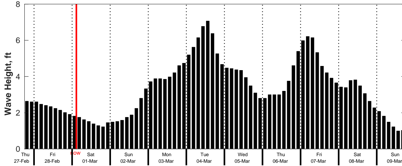
CMEMS Wave Forecast for NDBC 42092 from 27-Feb-2025 18:00:00 to 09-Mar-2025 18:00:00
