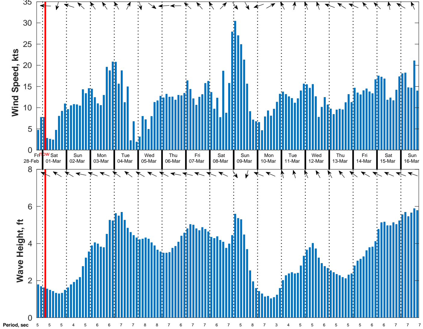
Wind & Wave Forecast for NDBC 42092 from 28-Feb-2025 18:00:00 to 16-Mar-2025 18:00:00
