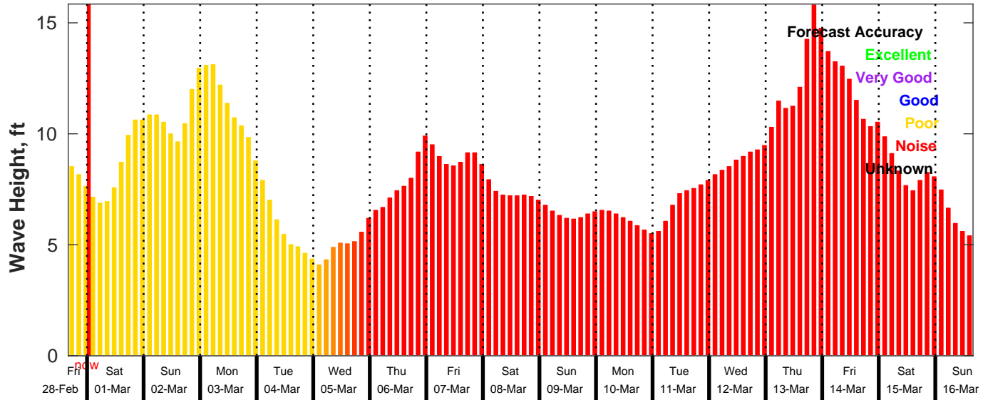
GFS Wave Forecast for NDBC 46011 from 28-Feb-2025 16:00:00 to 16-Mar-2025 16:00:00
