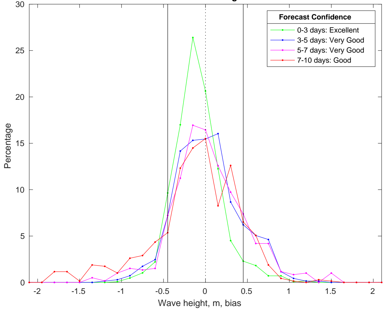
NDBC 46028 vs CMEMS Waves Bias Histogram: 01-Mar-2025
