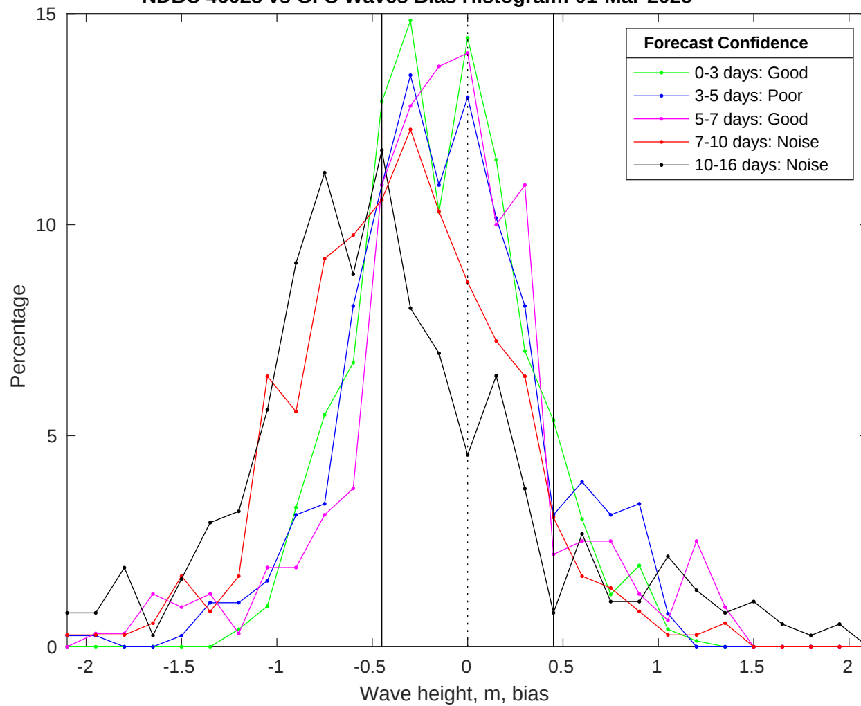
NDBC 46028 vs GFS Waves Bias Histogram: 01-Mar-2025
