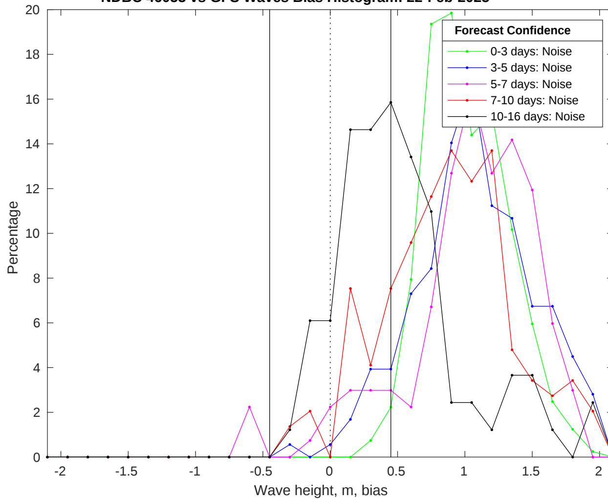
NDBC 46053 vs GFS Waves Bias Histogram: 22-Feb-2025
