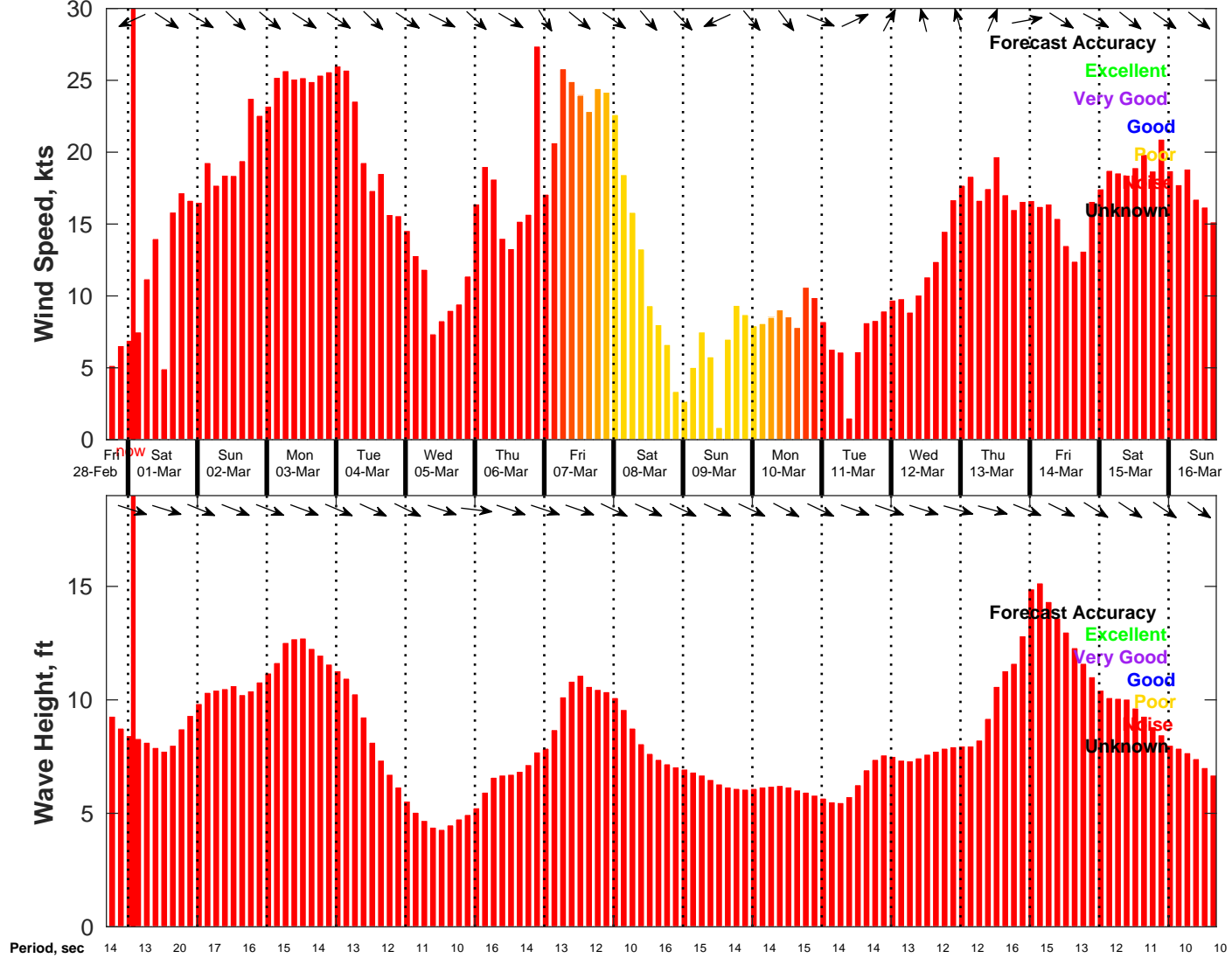
Wind & Wave Forecast for NDBC 46053 from 28-Feb-2025 17:00:00 to 16-Mar-2025 17:00:00
