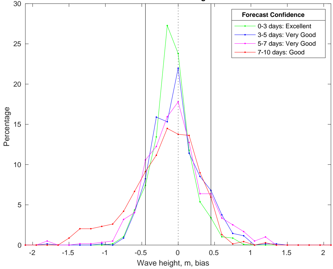
NDBC 46054 vs CMEMS Waves Bias Histogram: 01-Mar-2025
