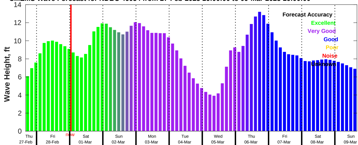
CMEMS Wave Forecast for NDBC 46054 from 27-Feb-2025 16:00:00 to 09-Mar-2025 16:00:00
