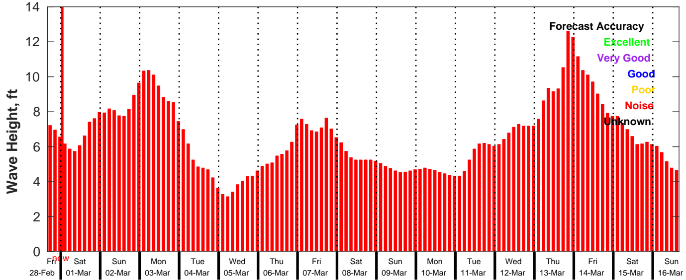
GFS Wave Forecast for NDBC 46054 from 28-Feb-2025 16:00:00 to 16-Mar-2025 16:00:00
