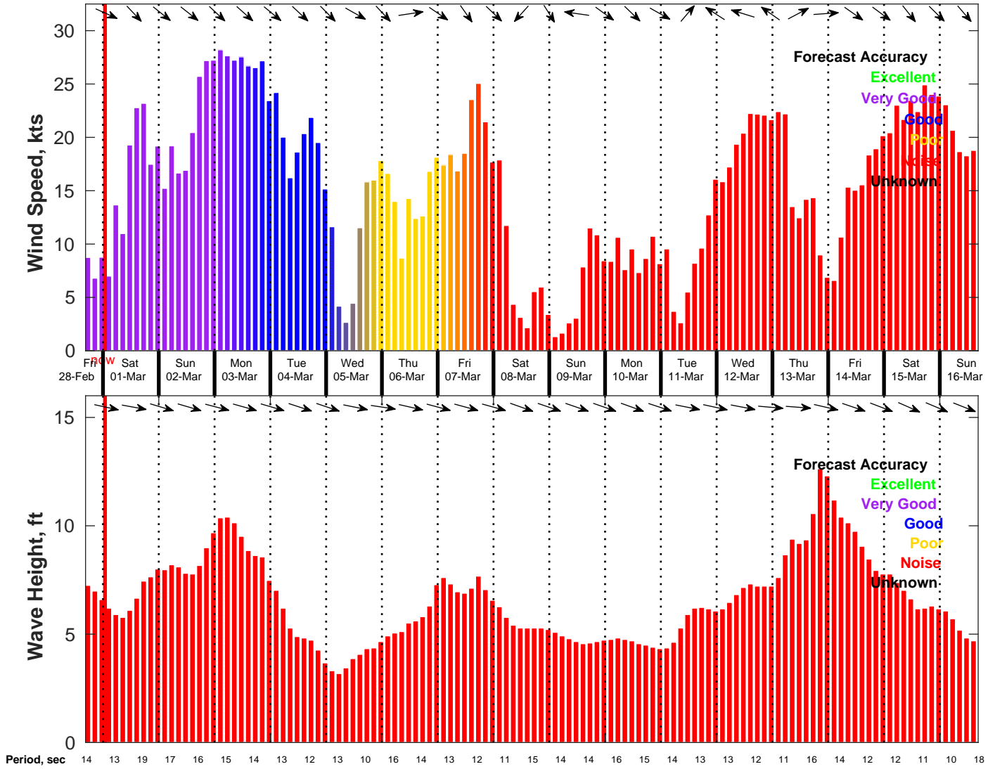
Wind & Wave Forecast for NDBC 46054 from 28-Feb-2025 16:00:00 to 16-Mar-2025 16:00:00
