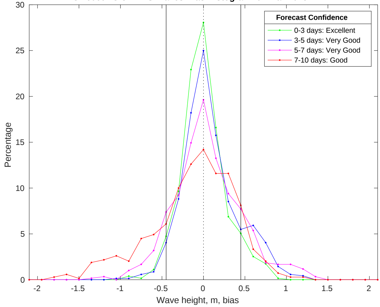
NDBC 46069 vs CMEMS Waves Bias Histogram: 01-Mar-2025
