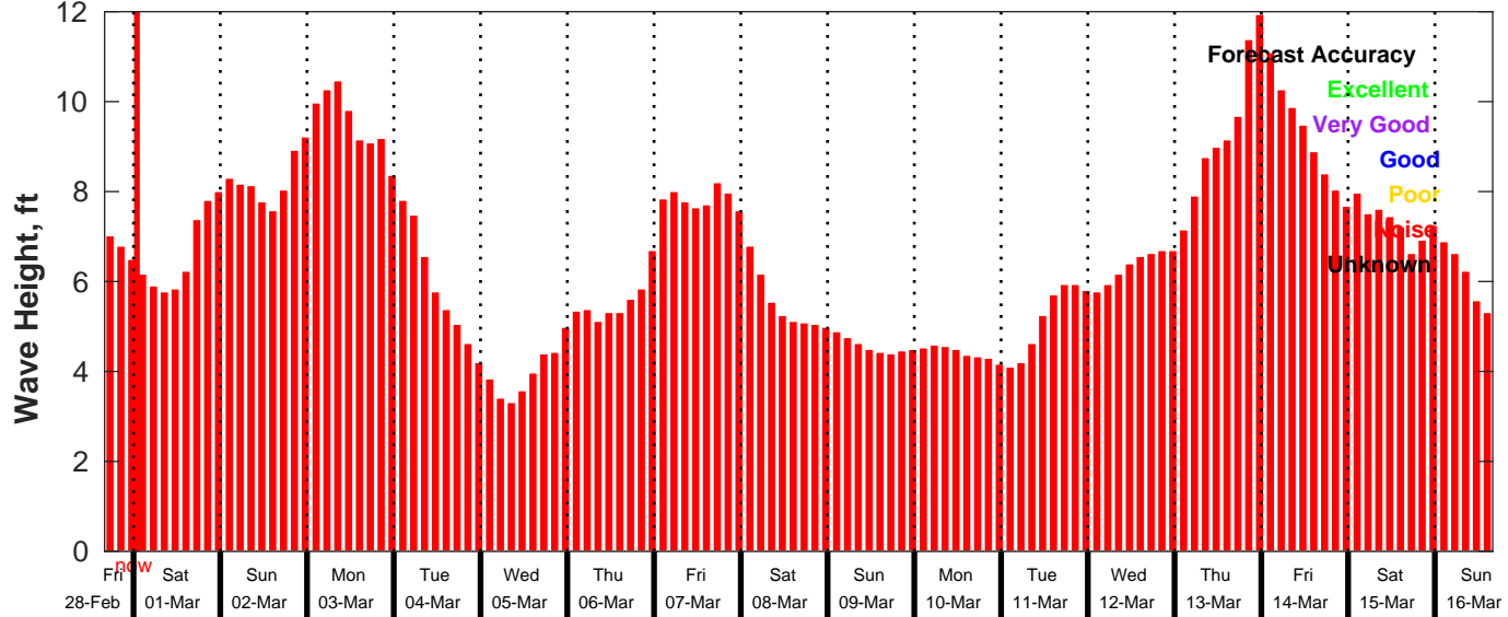
GFS Wave Forecast for NDBC 46069 from 28-Feb-2025 16:00:00 to 16-Mar-2025 16:00:00
