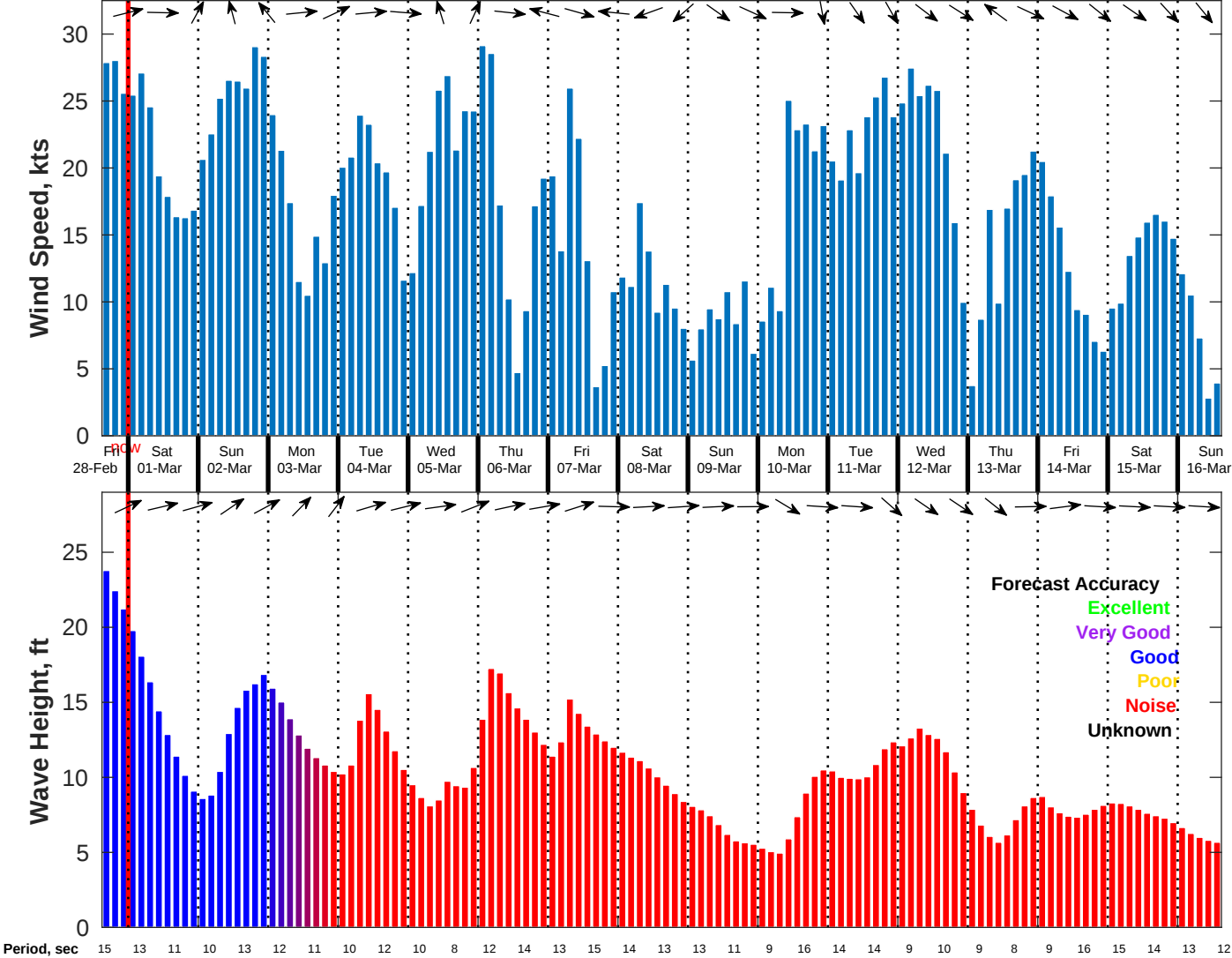
Wind & Wave Forecast for NDBC 46246 from 28-Feb-2025 15:00:00 to 16-Mar-2025 15:00:00
