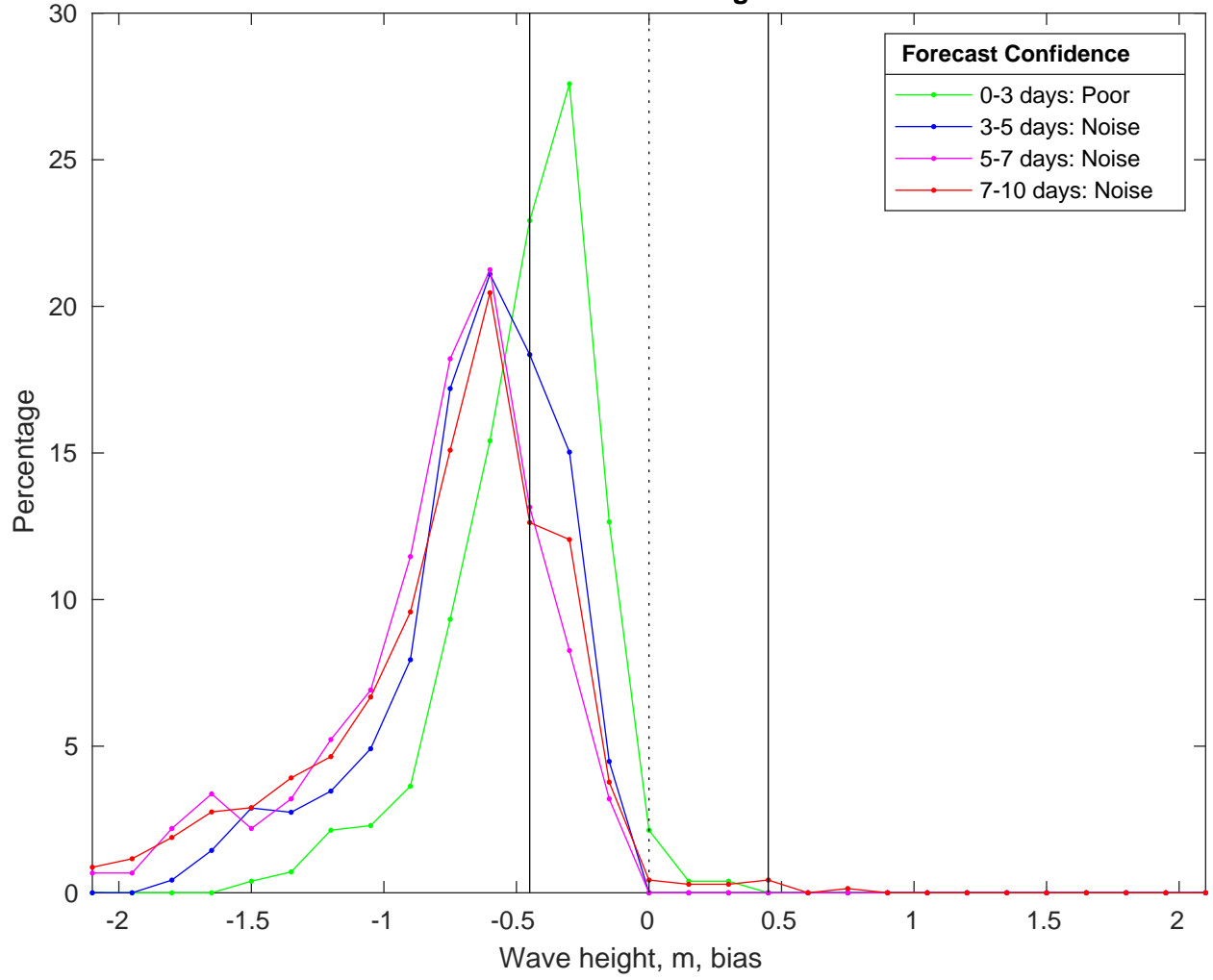
NDBC 51209 vs CMEMS Waves Bias Histogram: 01-Mar-2025
