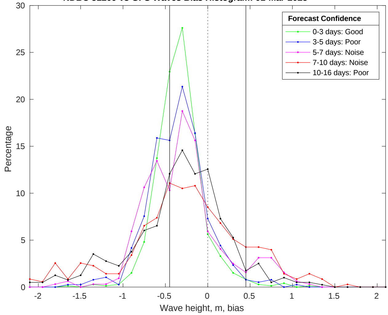
NDBC 51209 vs GFS Waves Bias Histogram: 01-Mar-2025
