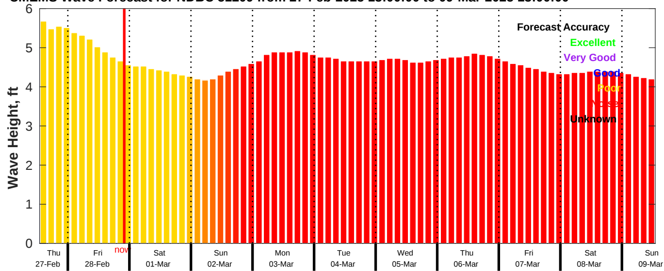
CMEMS Wave Forecast for NDBC 51209 from 27-Feb-2025 13:00:00 to 09-Mar-2025 13:00:00
