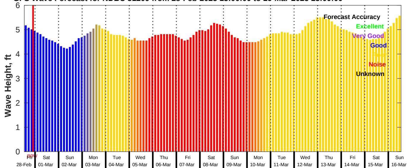
GFS Wave Forecast for NDBC 51209 from 28-Feb-2025 13:00:00 to 16-Mar-2025 13:00:00
