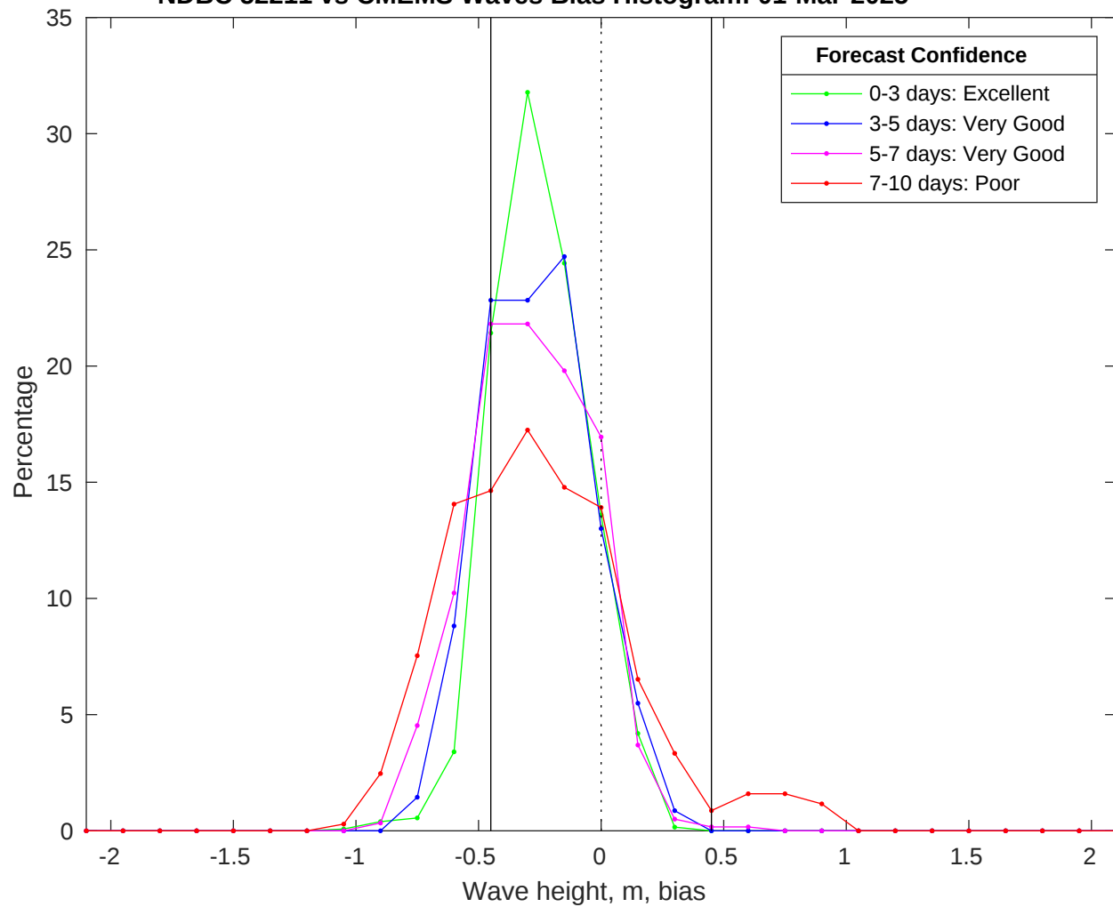
NDBC 52211 vs CMEMS Waves Bias Histogram: 01-Mar-2025
