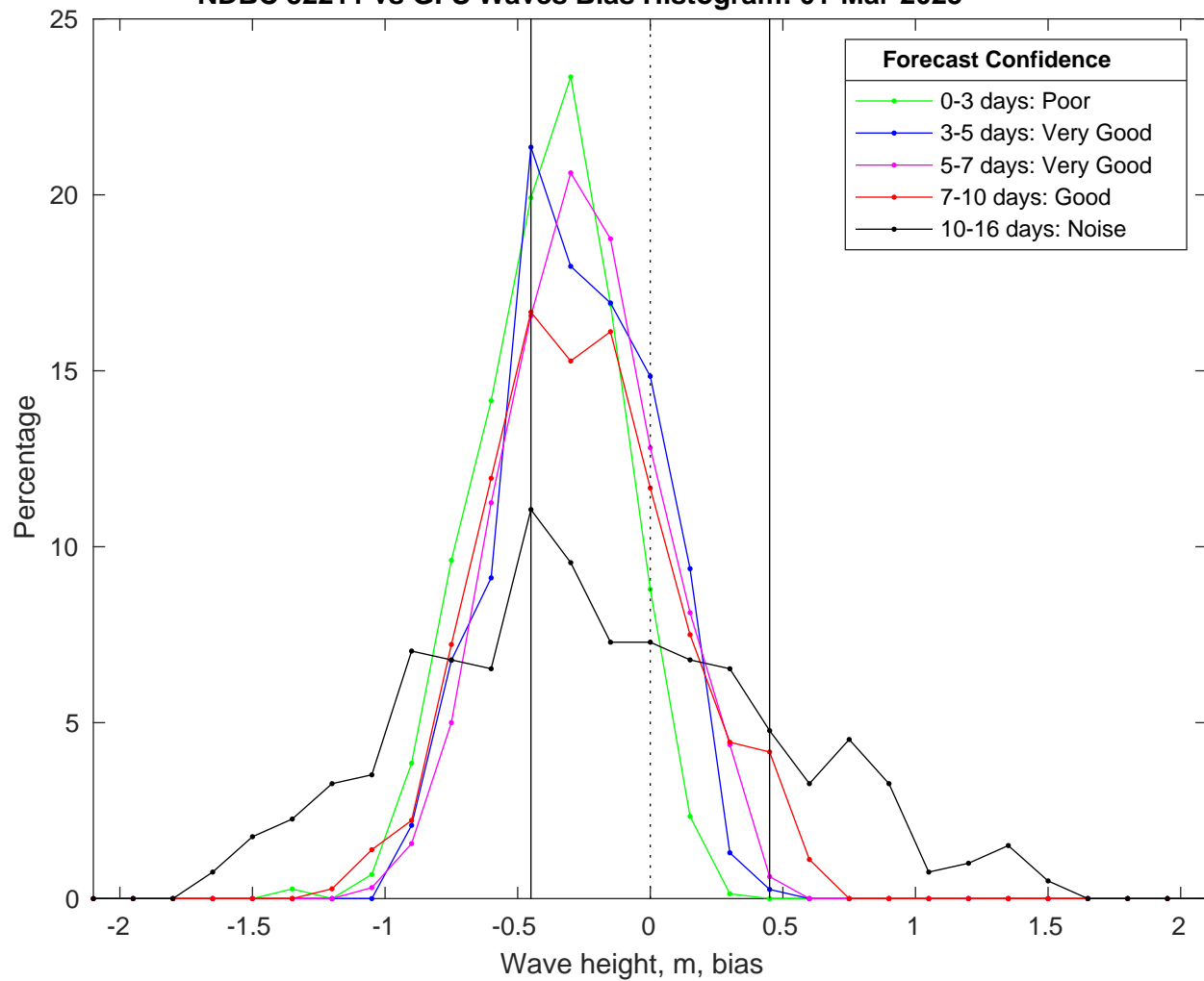
NDBC 52211 vs GFS Waves Bias Histogram: 01-Mar-2025
