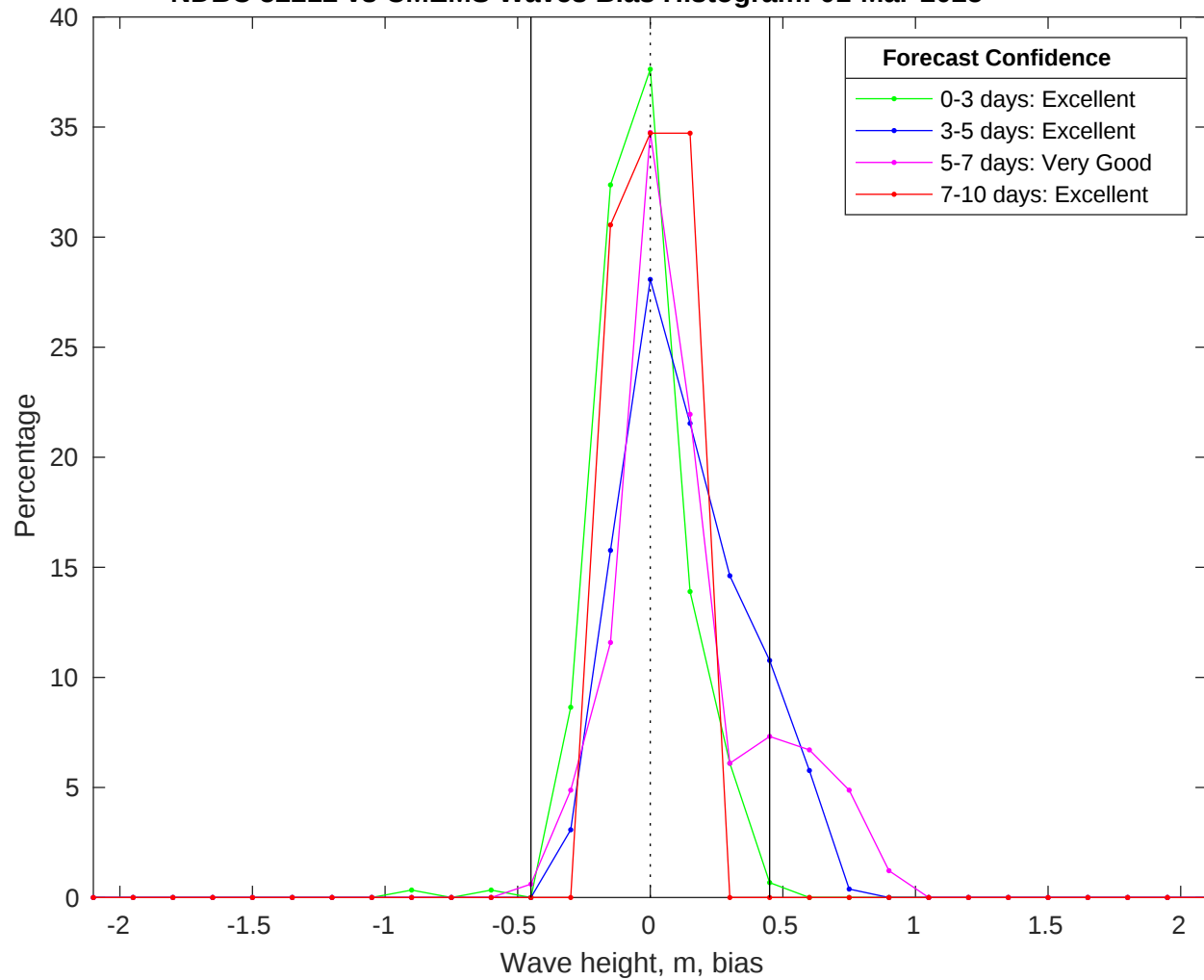
NDBC 52212 vs CMEMS Waves Bias Histogram: 01-Mar-2025
