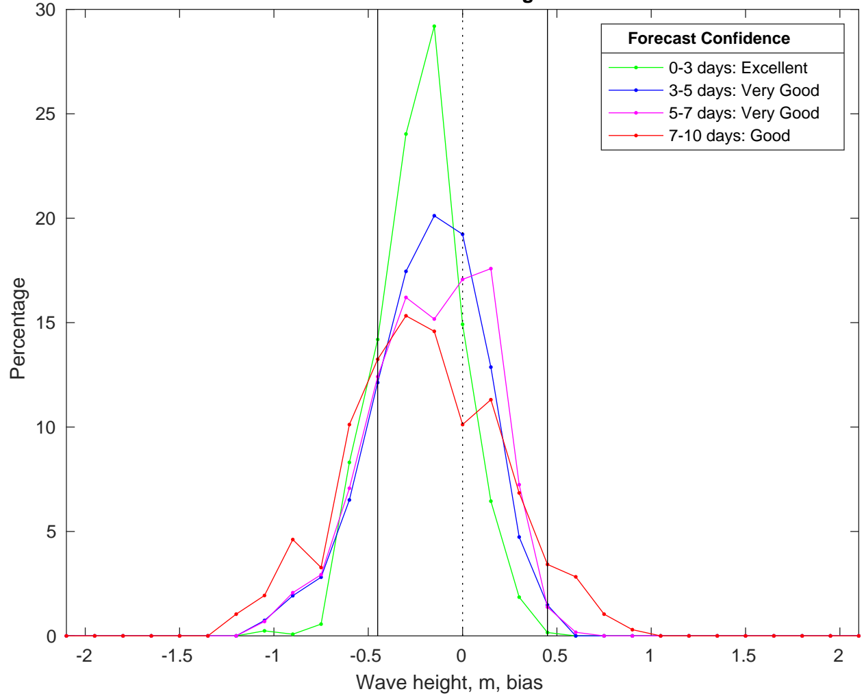
NDBC 52213 vs CMEMS Waves Bias Histogram: 01-Mar-2025
