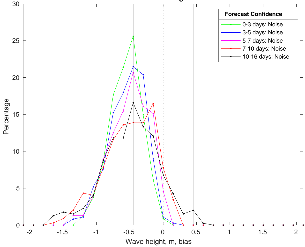
NDBC 52213 vs GFS Waves Bias Histogram: 01-Mar-2025
